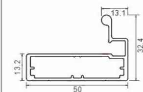
AVAP 1031 Aluminium Profile With Handle Size : 3000mm
