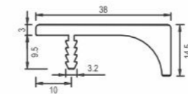
AVAP 1087 Aluminium Handle Profile Size : 3000mm
