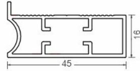
AVAP 1052 Aluminium Profile Size : 3000mm
