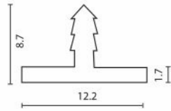
AVAP 1079 Aluminium Inlay Profile Size : 3000mm
