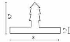
AVAP 1080 Aluminium Inlay Profile Size : 3000mm
