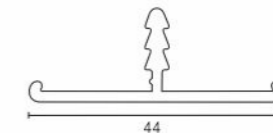
AVAP 057 Aluminium Edge Profile Size : 3000mm
