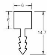
AVAP 1081 Aluminium Inlay Profile Size : 3000mm
