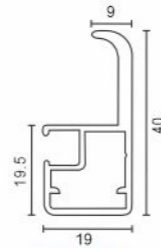
AVAP 058 Aluminium Profile With Handle Size : 3000mm
