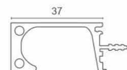
AVAP 1046 Aluminium Handle Profile Size : 3000mm
