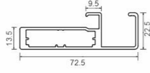
AVAP 077 Aluminium Profile With Handle For 6mm Glass Size : 3000mm
