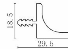
AVAP 1077 Aluminium Handle Profile Size : 3000mm
