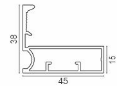
AVAP 1057 Aluminium Handle Profile Size : 3000mm
