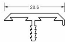
AVAP 1082 Aluminium Edge Profile Size : 3000mm
