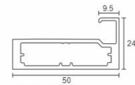
AVAP 043 Aluminium Profile For 8mm Glass Size : 3000mm
