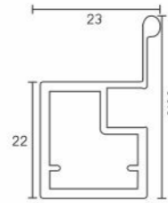
AVAP 030 Aluminium Profile With Handle Size : 3000mm
