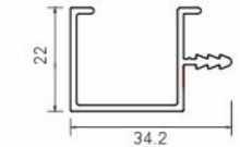
AVAP 1068 Aluminium Handle Profile Size : 3000mm
