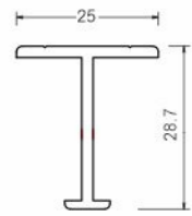
AVAP 1092 Aluminium Handle Profile Size : 3000mm
