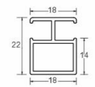
AVAP 1004 I Aluminium 'I' Profile For 4mm Glass Size : 3000mm
