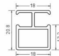
AVAP 1005 I Aluminium 'I' Profile For 4mm Glass Size : 3000mm
