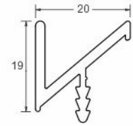
AVAP 1075 Aluminium Handle Profile Size : 3000mm
