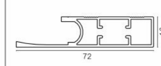
AVAP 1051 Aluminium Handle Profile Size : 3000mm
