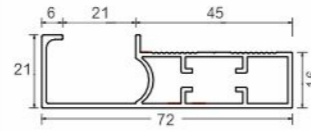
AVAP 1054 Aluminium Handle Profile Size : 3000mm
