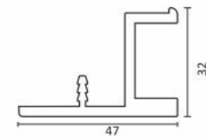
AVAP 1096 Aluminium Handle Profile Size : 3000mm
